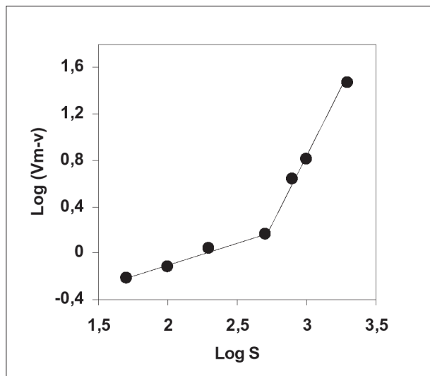
Figure 1. Hill plot of pure rat intestinal BChE with BTCh. Initial velocities were determined in the activity mixture containing 100 mM MOPS buffer, pH 7.4, 0.250 mM DTNB, 0–50 mM BTCh, and 3.65 µg/ml pure enzyme.
