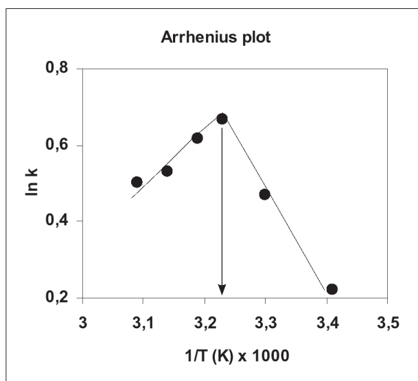
Figure 2. The graph of 1/T versus \ln k , the rate constant for different temperatures in which the slope is equal to -E_a/R . Sudden drop in the plot indicates enzyme inactivation. Arrow indicates that optimum temperature of the enzyme is 37°C (310 K). Initial velocities were determined in the activity mixture containing 100 mM MOPS buffer, pH 7.4, 0.250 mM DTNB, 4 mM BTCh, and 3.65 µg/ml pure enzyme.
