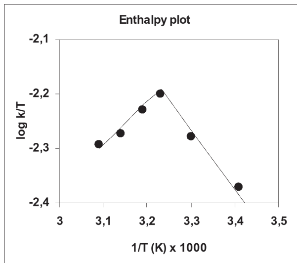
Figure 3. \Delta H was determined by measuring the rate constant ( k ) at several different temperature and plotting \log k/T versus 1/T . The slope = \Delta H / 2.3 R . Initial velocities were determined in the activity mixture containing 100 mM MOPS buffer, pH 7.4, 0.250 mM DTNB, 4 mM BTCh, and 3.65 µg/ml pure enzyme.
